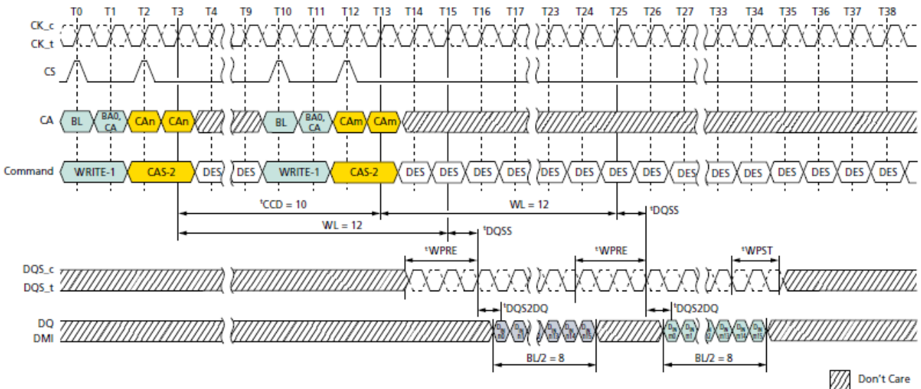
Consecutive WRITE: t'_{CCD} = \text{MIN} + 2, 1.5n\text{CK} Postamble
