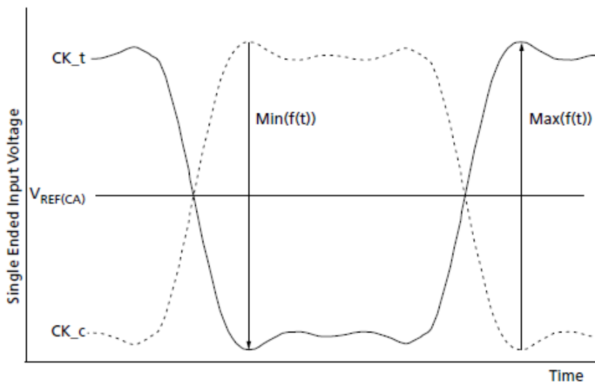
Definition of Differential Clock Peak Voltage
