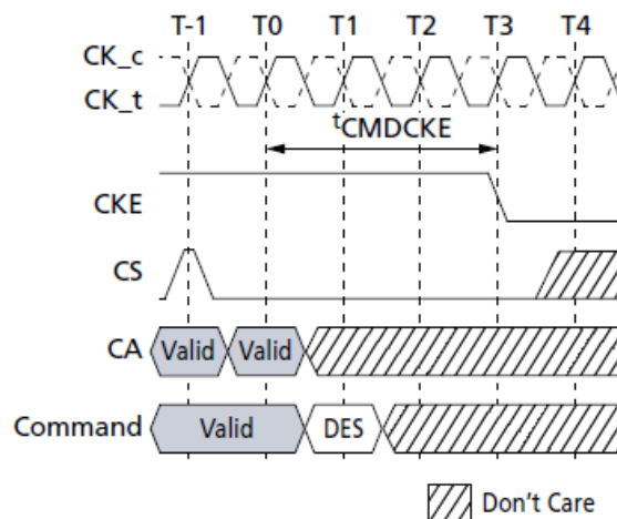
t_{CMDCKE} Timing
