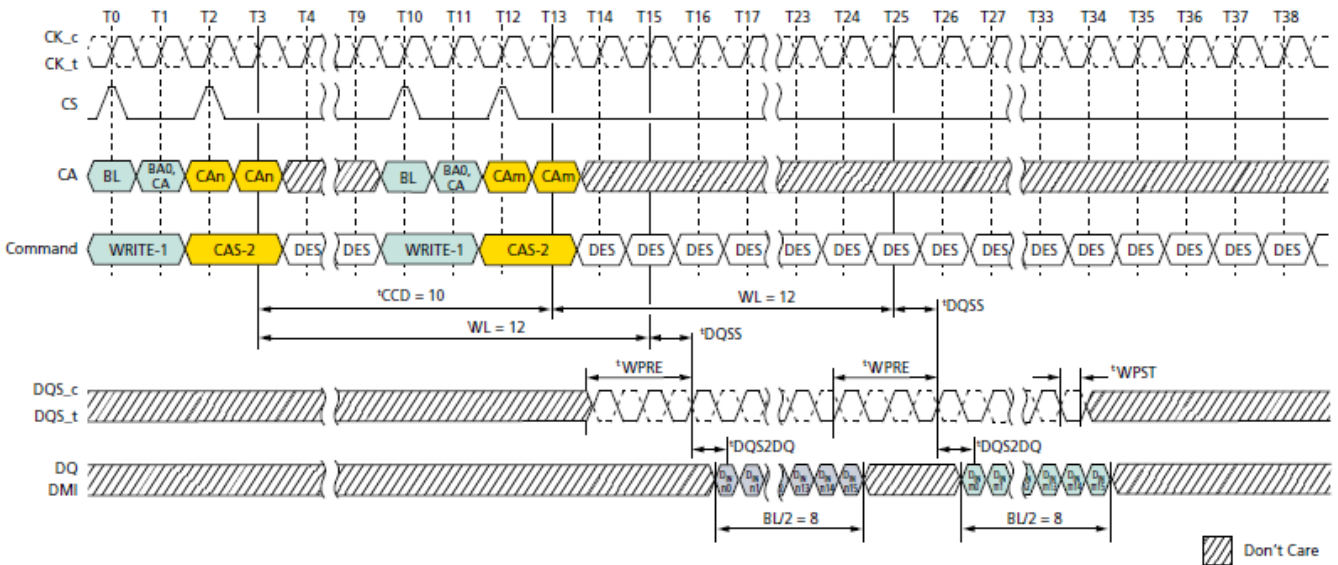
Consecutive WRITE: t'_{CCD} = \text{MIN} + 2, 0.5n\text{CK} Postamble
