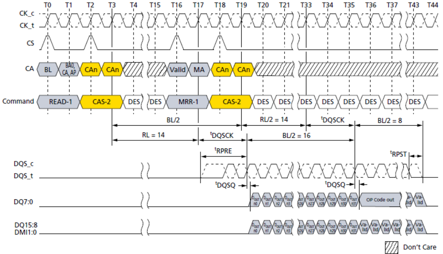
READ-to-MRR Timing
