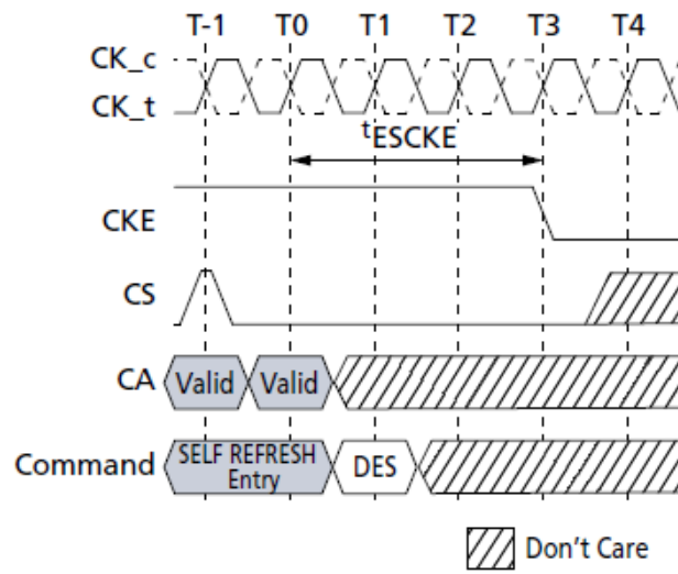
t_{ESCKE} Timing
