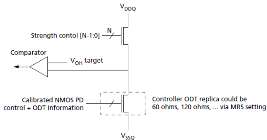
Pull-Up Calibration
