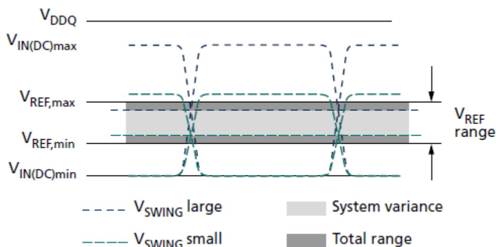
V_{REF} Operating Range ( V_{REF,max} , V_{REF,min} )
