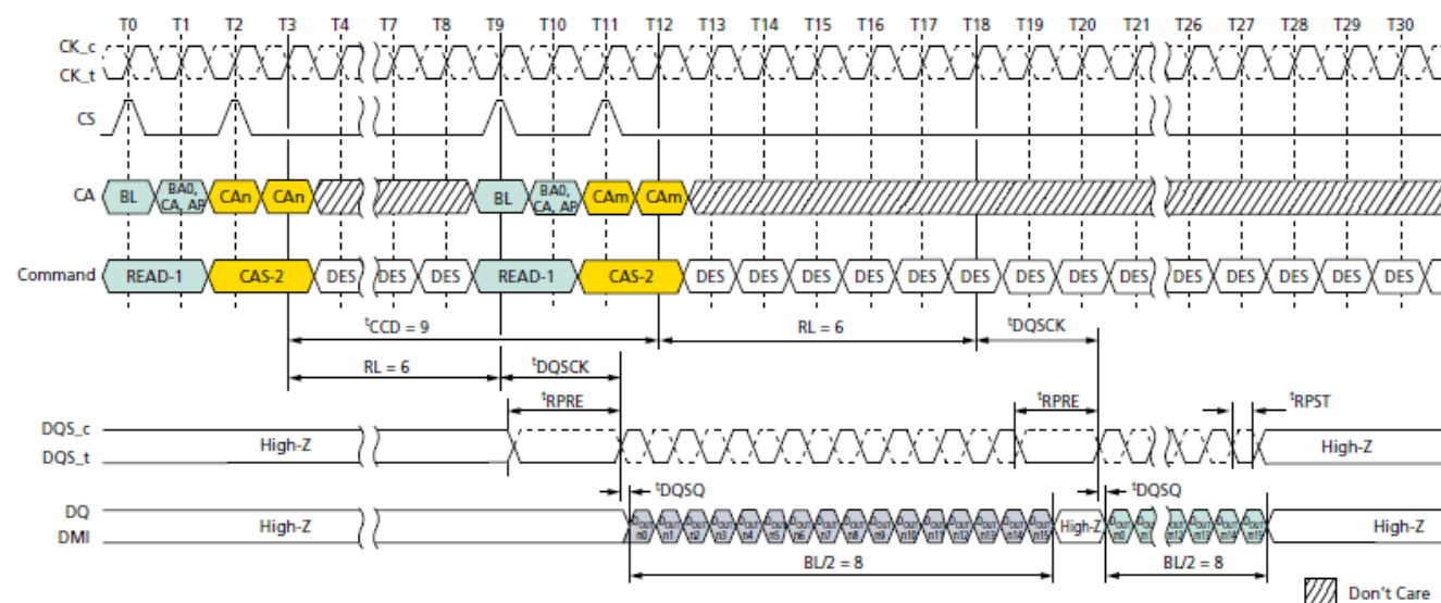
Consecutive READ: t_{CCD} = \text{MIN} + 1 , Preamble = Static, 0.5n\text{CK} Postamble
