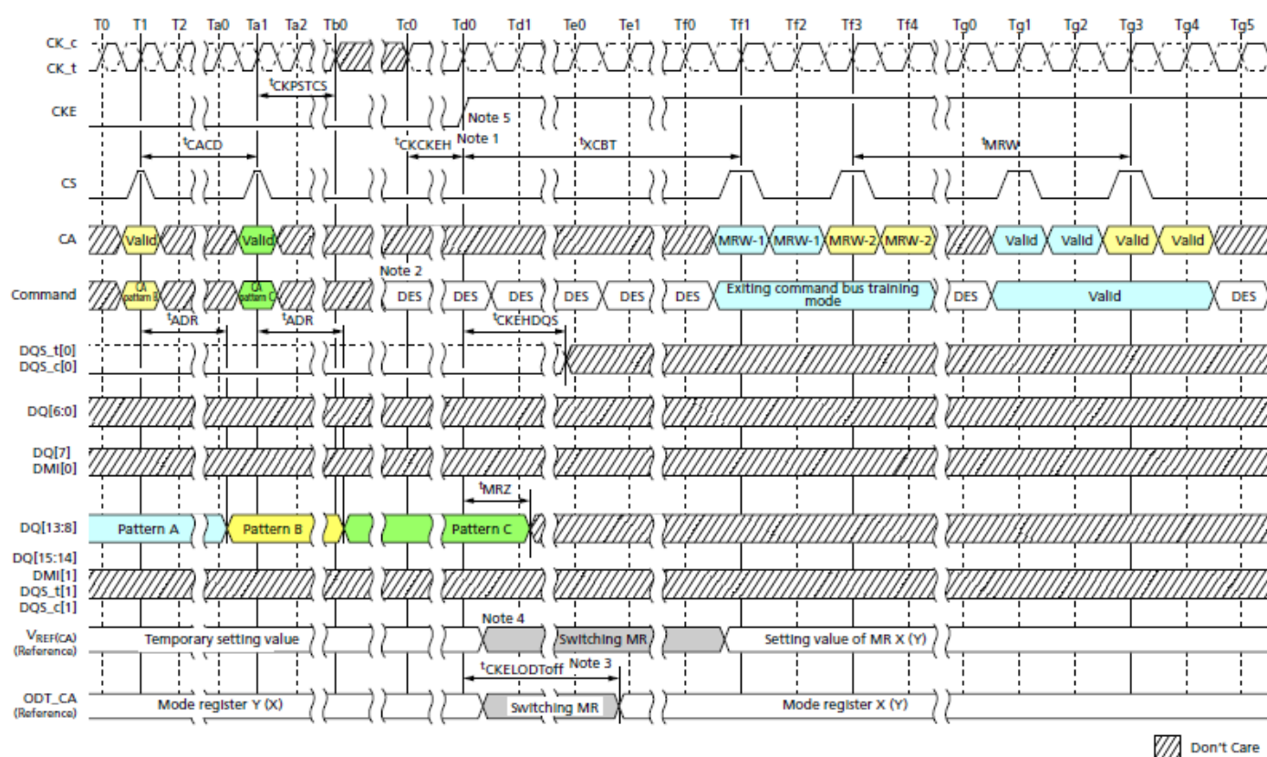
Command Bus Training Mode Exit with Valid Command
