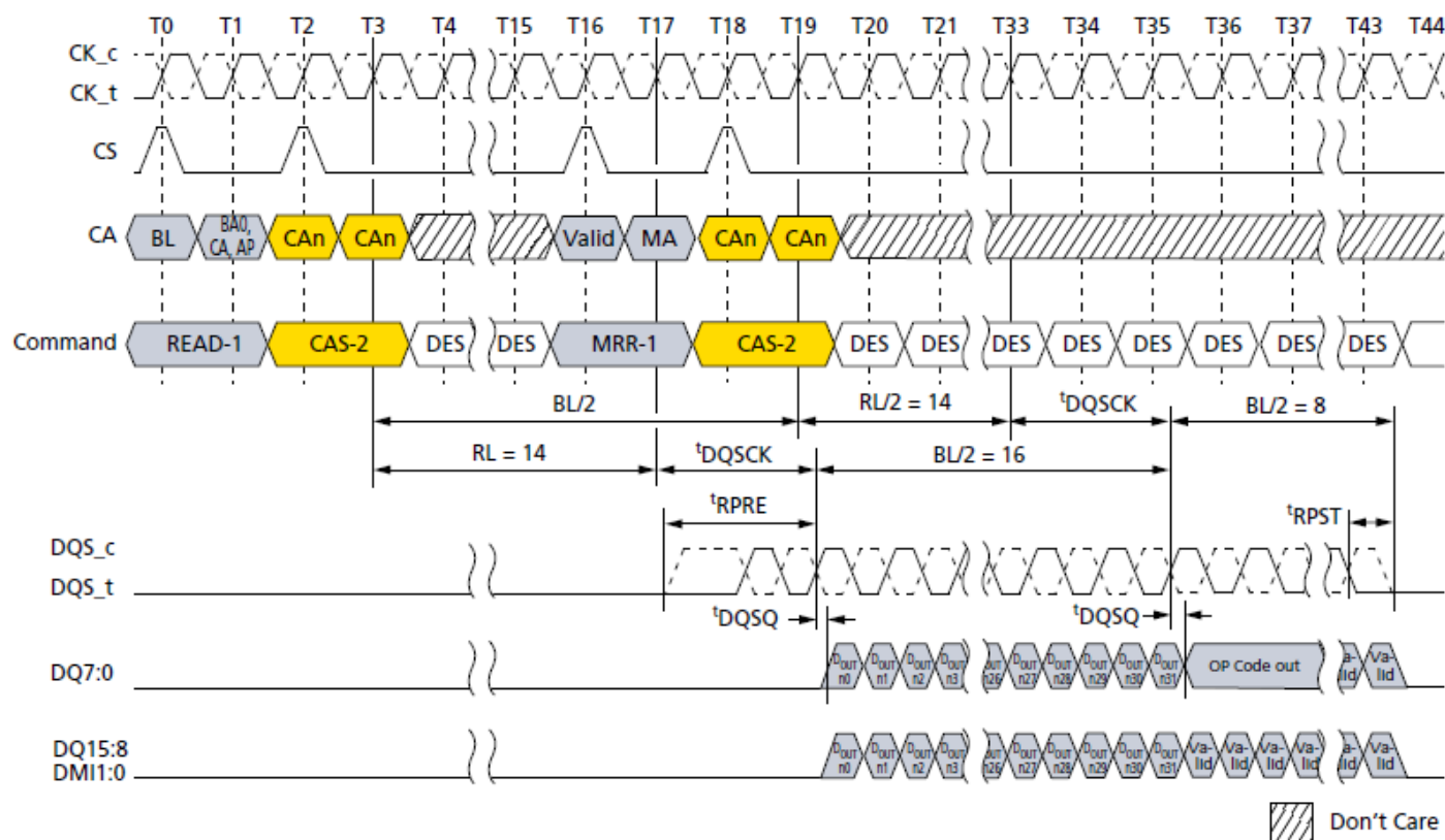
READ-to-MRR Timing
