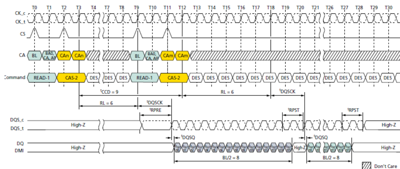
Consecutive READ: t_{CCD} = \text{MIN} + 1 , Preamble = Static, 1.5n\text{CK} Postamble
