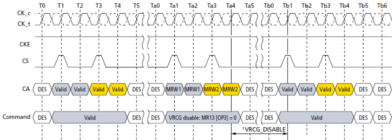
VRCG Disable Timing
