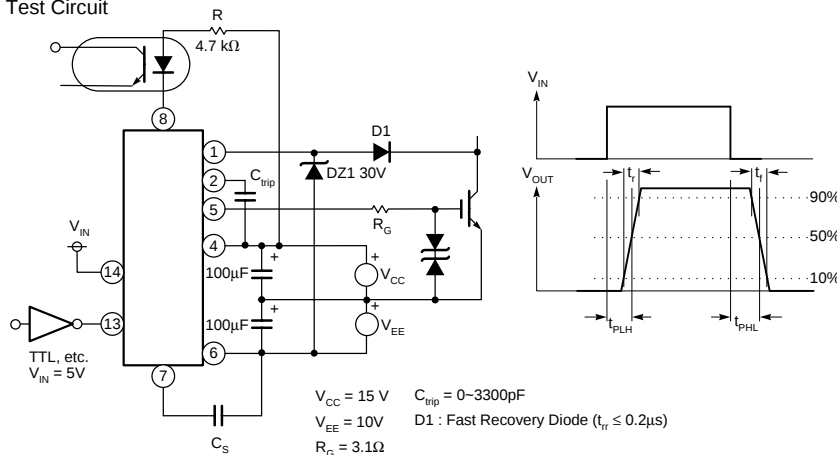
Test Circuit
