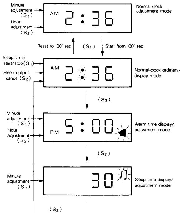
Note 5: The symbol \text{⌘} shows a 2sec-period on-off flash 6: Lock switches are used in the S_4 and S_5 pins.
