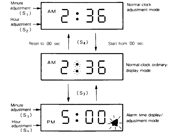
Note 3: The symbol \text{⌘} shows a 2sec-period on-off flash 4: Lock switches are used in the S_3 , S_4 and S_5 pins
