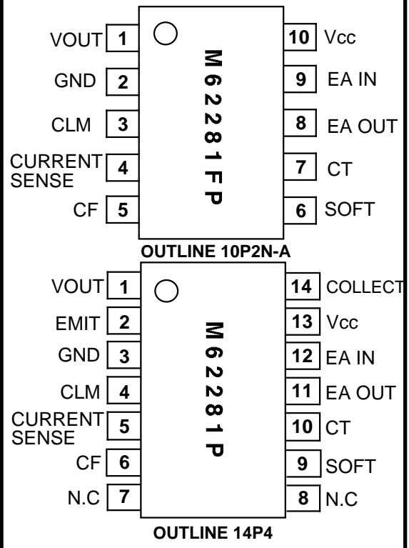
PIN CONFIGURATION (TOP VIEW)
