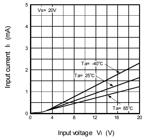
Input Characteristics
