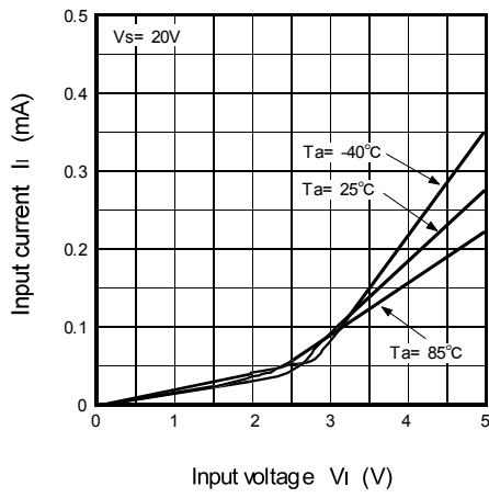
Input Characteristics
