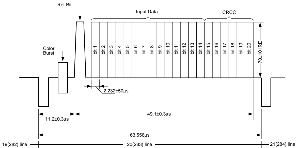
Fig. 2 CGMS WAVEFORM
