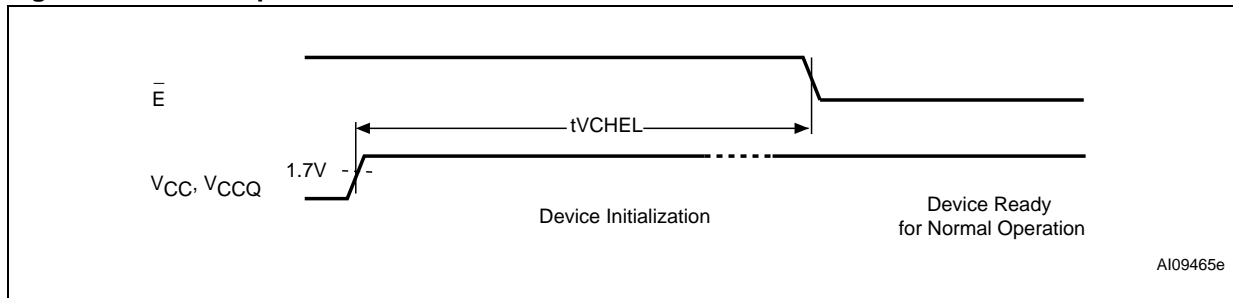
Figure 27. Power-Up AC waveforms
