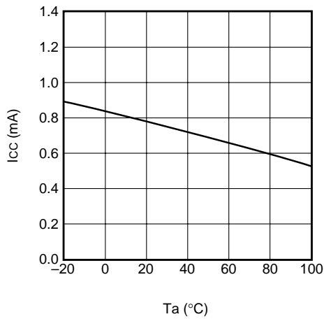
Icc vs. Temperature
