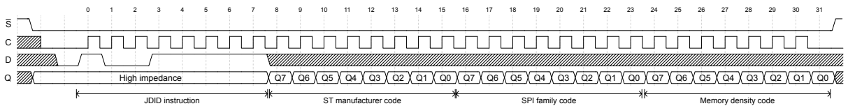
Figure 29. JEDEC identification
