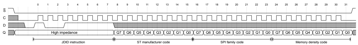
Figure 29. JEDEC identification
