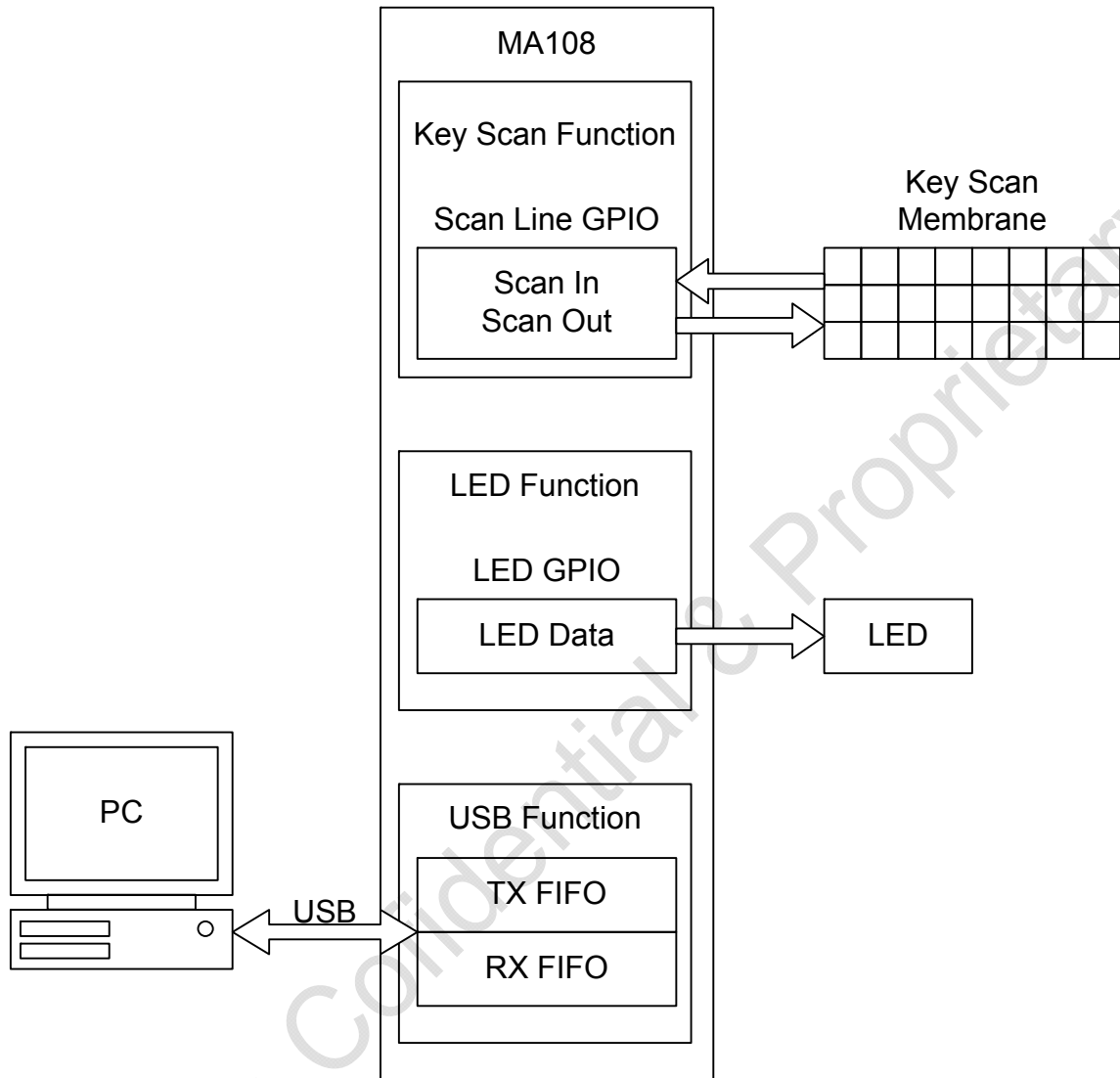
Figure 3-1 Keyboard Diagram
