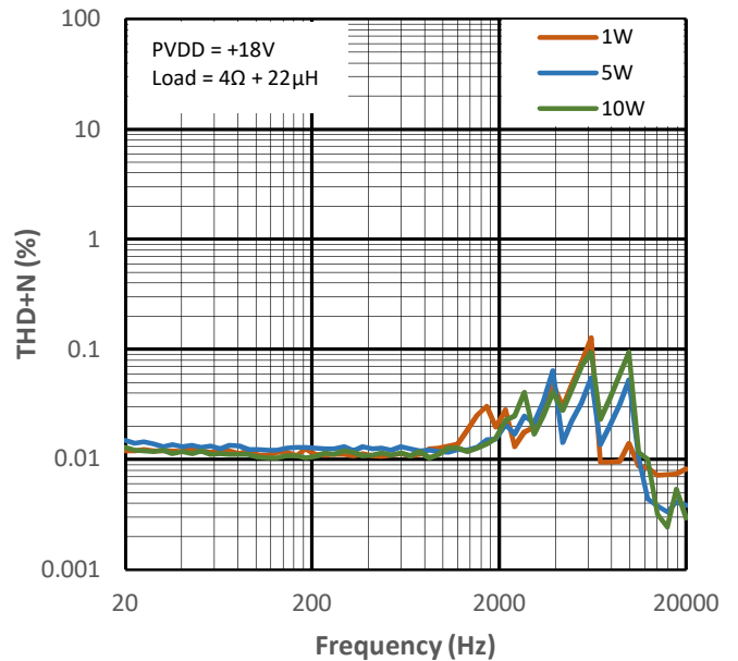
Figure 10-8 THD+N vs Frequency for PMP4
