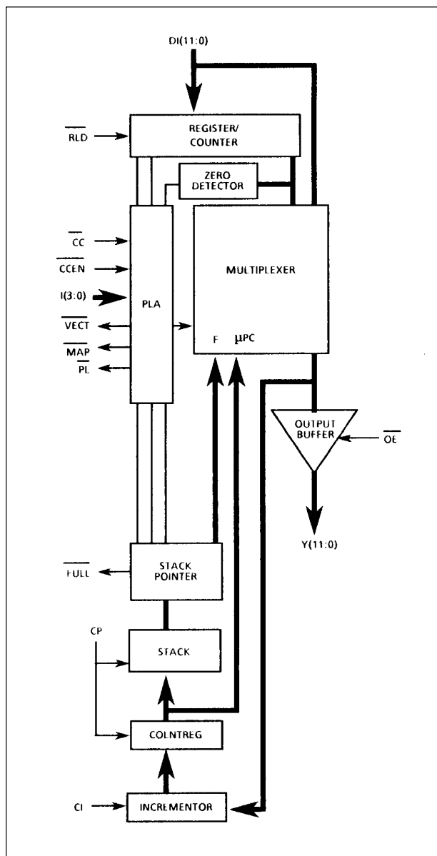
Figure 1: Block Diagram
