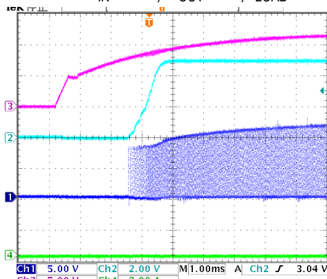
Cable On : V_{IN} = 12V, V_{OUT} = 5V, I_{LOAD} = 2A
