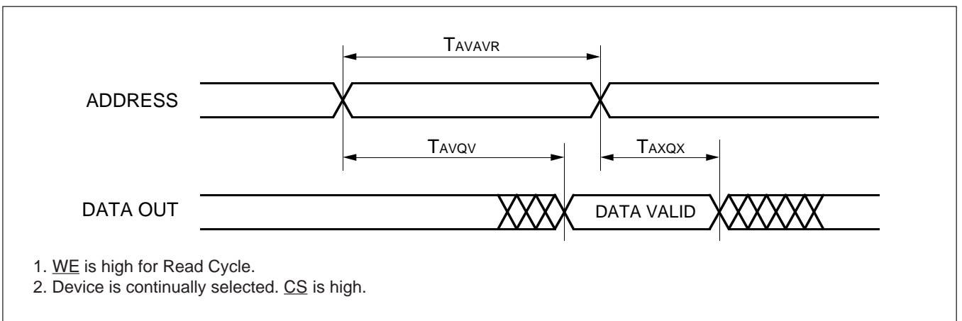
Figure 11b: Read Cycle 2
