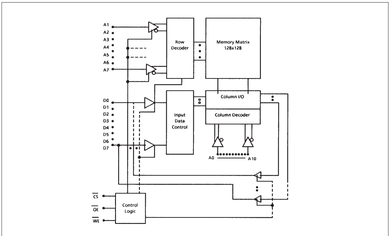
Figure 2: Block Diagram
