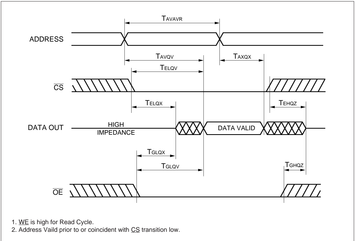
Figure 11a: Read Cycle 1
