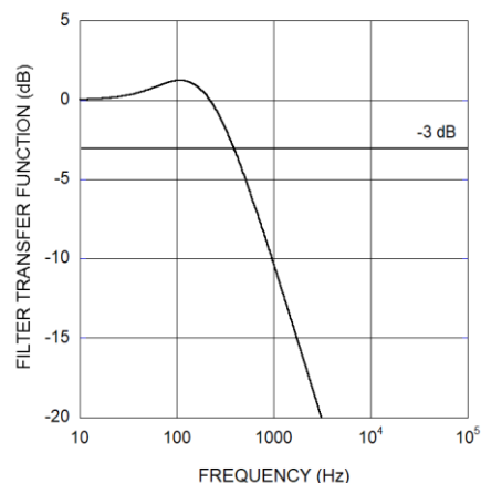
Filter Transfer Function vs. Frequency
