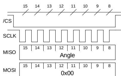
Figure 11: Partial 8-Bit SPI Angle Reading
