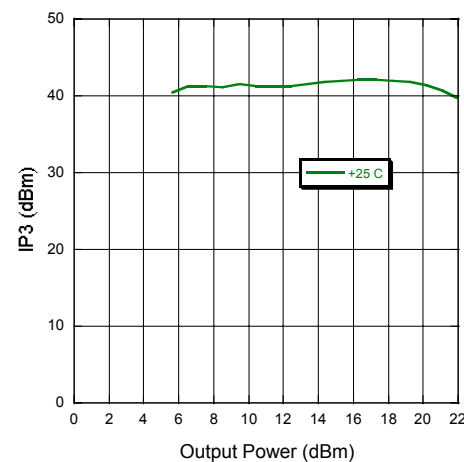
Output IP3
