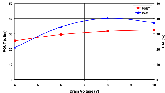
Figure 2. Saturated Output Power and Power Added Efficiency vs. Drain Voltage at f_0 = 7\text{ GHz} .
