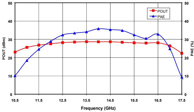
Figure 1. Output Power and Power Added Efficiency vs. Frequency at V_{DD} = 8V and P_{in} = 12\text{ dBm} .
