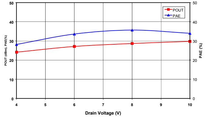
Figure 2. Saturated Output Power and Power Added Efficiency vs. Drain Voltage at f_o = 14\text{ GHz} .
