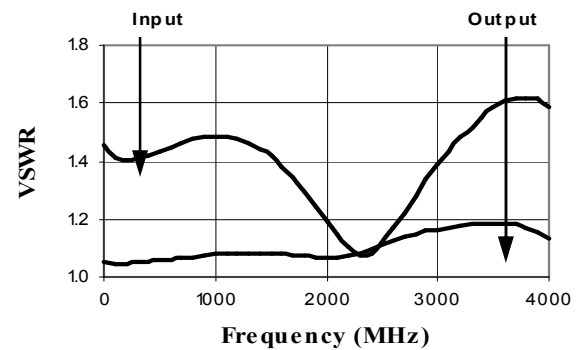
VSWR, 8 dB Bit
