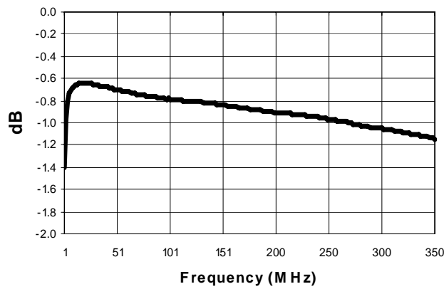
Amplitude Unbalance
