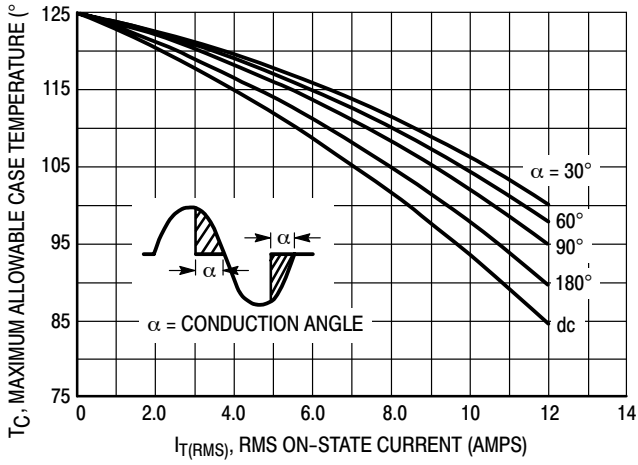
Figure 1. Current Derating
