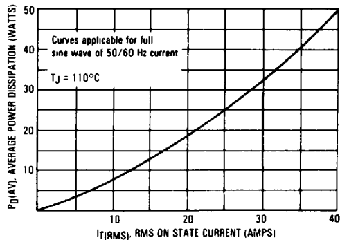
FIGURE 5 — ON-STATE POWER DISSIPATION
