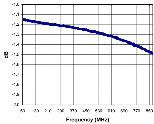
Return Loss: Input port
