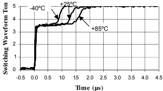
RX Off, 20 mA Load Current
