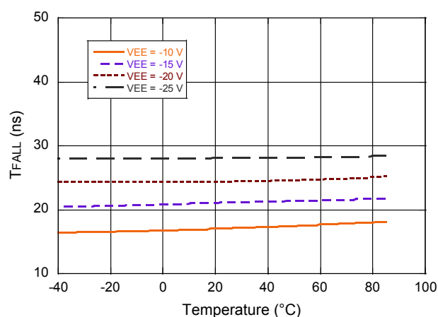
Switching Speed Driving 100 pF Capacitor: T_{FALL}
