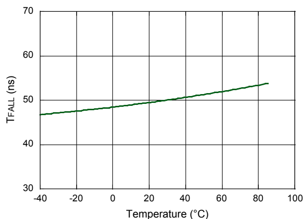
Switching Speed Driving MASW-002103: T_{FALL}
