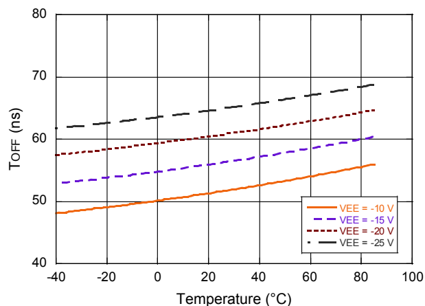
Switching Speed Driving 100 pF Capacitor: T_{OFF}
