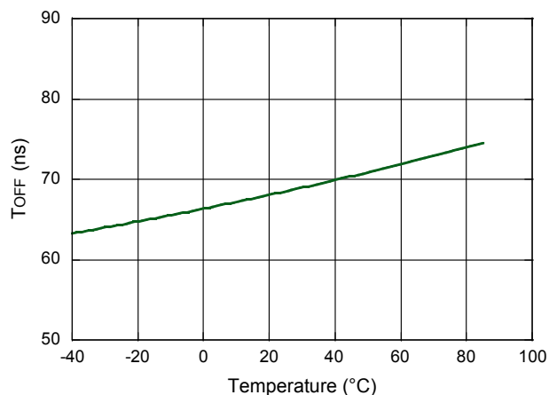
Switching Speed Driving MASW-002103: T_{OFF}
