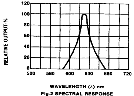
Fig. 2 SPECTRAL RESPONSE
