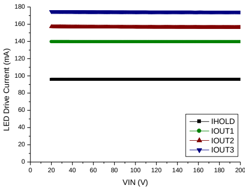
LED Drive current Vs. Input Voltage
