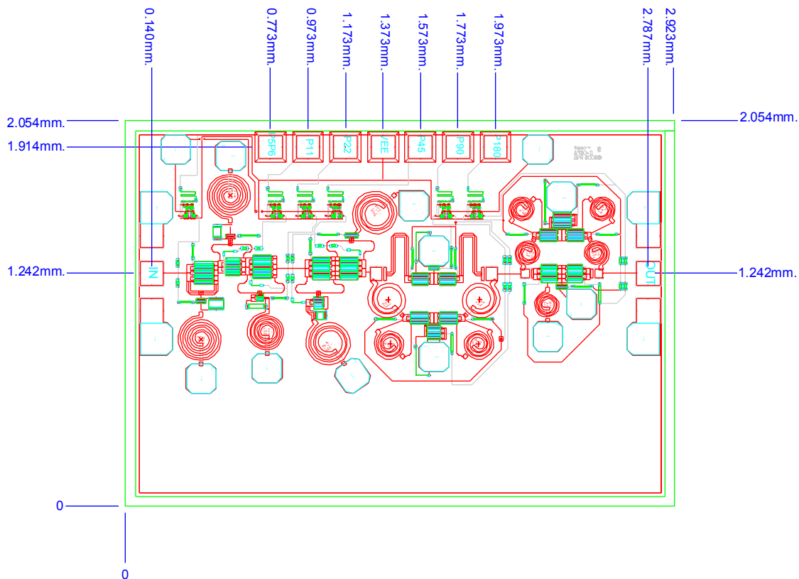
Figure 7. Die Layout
