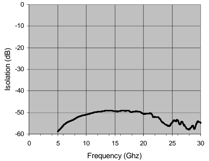
TYPICAL ISOLATION
