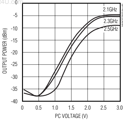
MODULATOR OUTPUT POWER vs. PC VOLTAGE (ENX2 = GND)
