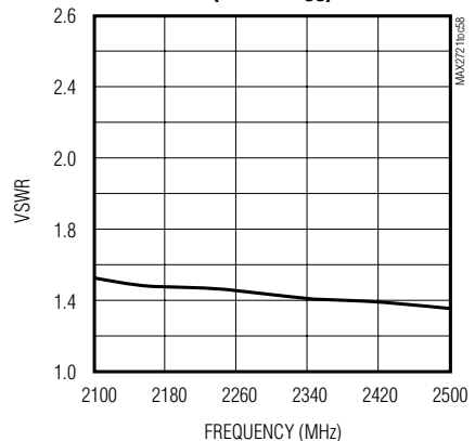
LO PORT VSWR vs. LO FREQUENCY ( ENX2 = V_{CC} )
