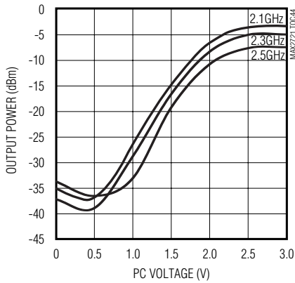
MODULATOR OUTPUT POWER vs. PC VOLTAGE (ENX2 = VCC)
