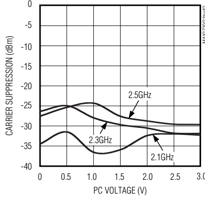
CARRIER SUPPRESSION vs. PC VOLTAGE (ENX2 = GND)
