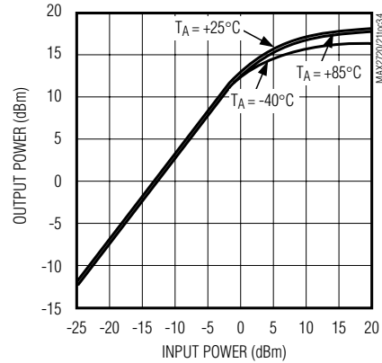
PA DRIVER OUTPUT POWER vs. INPUT POWER
