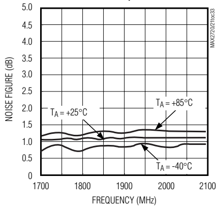
PA DRIVER NOISE FIGURE vs. FREQUENCY
