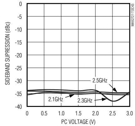
SIDEBAND SUPPRESSION vs. PC VOLTAGE (ENX2 = GND)
