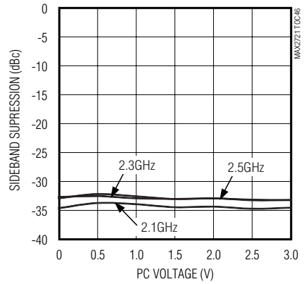
MODULATOR SIDEBAND SUPPRESSION vs. PC VOLTAGE (ENX2 = VCC)
