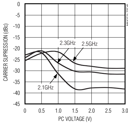
MODULATOR CARRIER SUPPRESSION vs. PC VOLTAGE (ENX2 = VCC)
