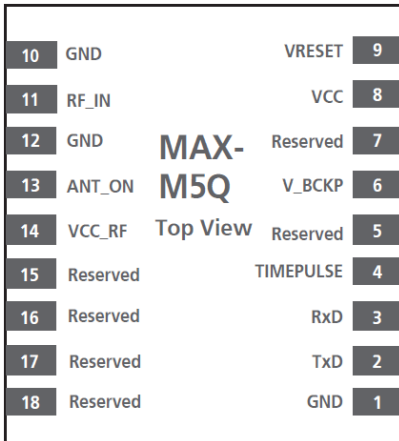
Figure 4: Pin Assignment of MAX-M5Q
