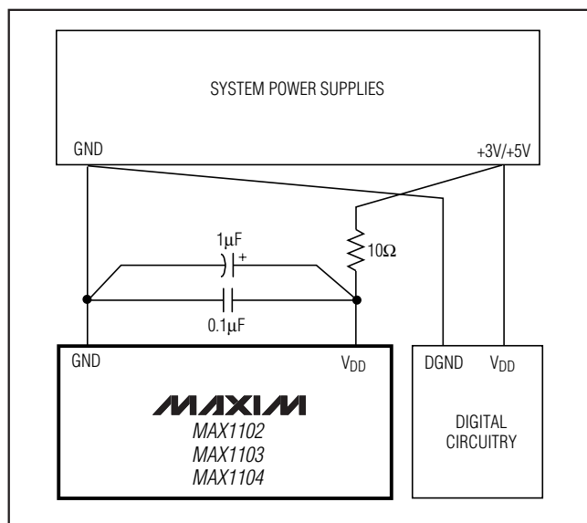
Figure 10. Power-Supply Connections
