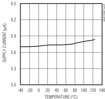
VS SUPPLY CURRENT vs. TEMPERATURE (SHUTDOWN MODE)
