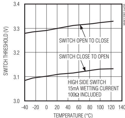
SWITCH THRESHOLD vs. TEMPERATURE (HIGH SIDE SWITCH)
