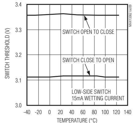
SWITCH THRESHOLD vs. TEMPERATURE (LOW-SIDE SWITCH)
