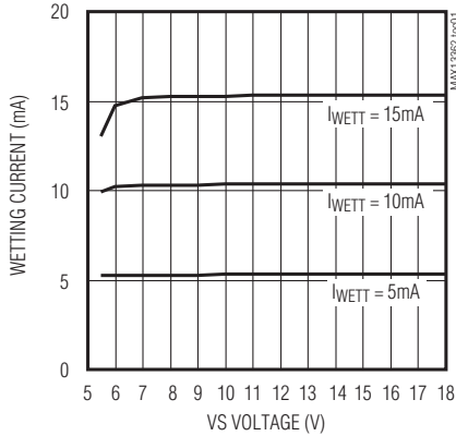
WETTING CURRENT (POLLING MODE)
