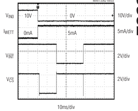
SWITCH STATUS CHANGE (CONTINUOUS MODE)
