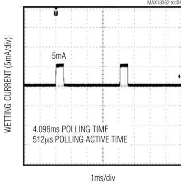
WETTING CURRENT (POLLING MODE)
