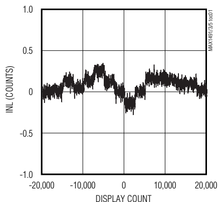
MAX1493/MAX1495 ( \pm 200mV INPUT RANGE) INL vs. DISPLAY COUNT
