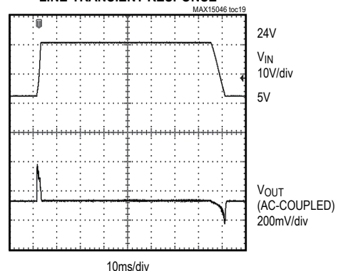
LINE-TRANSIENT RESPONSE
