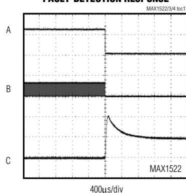
FAULT-DETECTION RESPONSE
