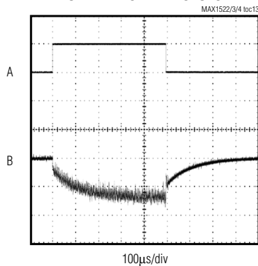
LOAD-TRANSIENT RESPONSE
