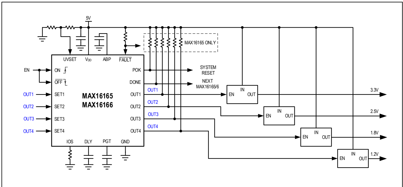
Figure 7. Sequence Four Power Supplies, without Monitoring. Only Monitor V_{DD} .
