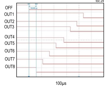
DAISY-CHAINING TWO DEVICES WITH EN RISING (CDLY = CPGT = OPEN)
