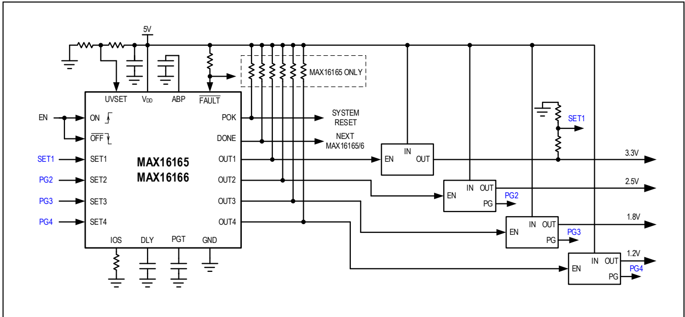
Figure 6. Sequence Four Power Supplies, Monitor V_{DD} , V_1 = 3.3V , and Power-Good Signals of the Other Three Power Supplies.
