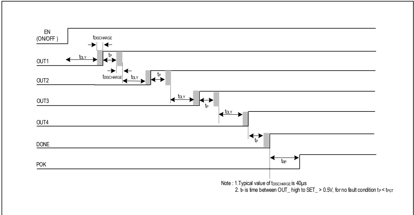
Figure 8. Power-Up Sequencing Timing Diagram. See the Typical Application Circuit (Figure 3).
