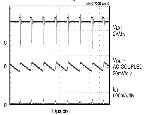
REG1 LIGHT-LOAD SWITCHING WAVEFORM LOAD = 10mA, V_{IN} = 4\text{V}
