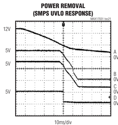
A. INPUT VOLTAGE, 5V/div C. 5V SMPS, 2V/div B. 5V LDO OUTPUT, 2V/div D. PGOOD, 5V/div
