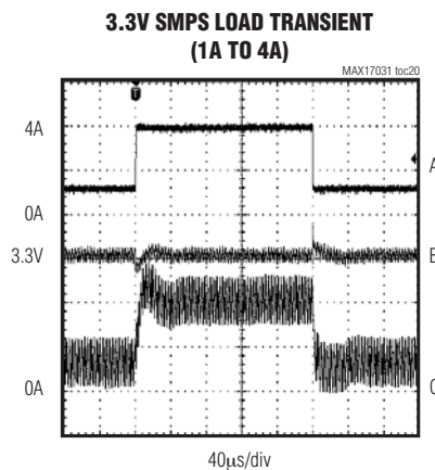
A. LOAD CURRENT, 2A/div C. INDUCTOR CURRENT, 100mV/div B. 3.3V SMPS OUTPUT, 2A/div
