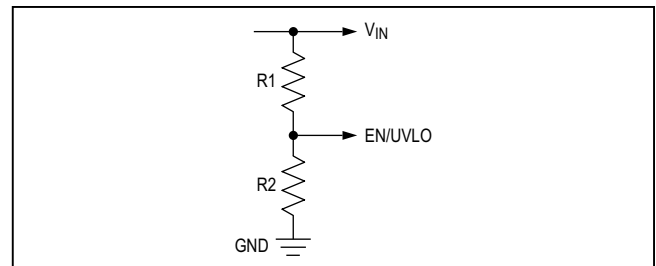
Figure 2. Adjustable EN/UVLO Network
