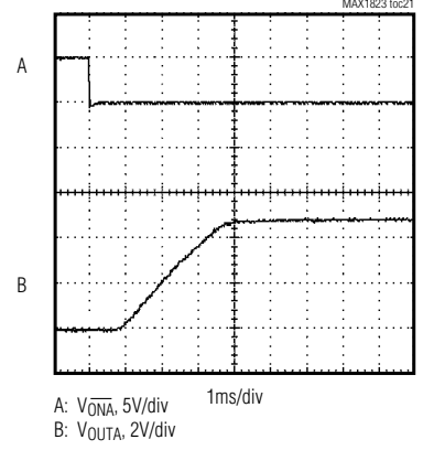
SWITCH TURN-ON TIME (MAX1823/MAX1823A)
