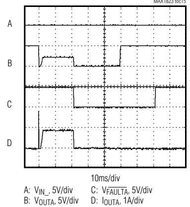
SHORT-CIRCUIT RESPONSE INTO 0Ω (MAX1823/MAX1823H)
