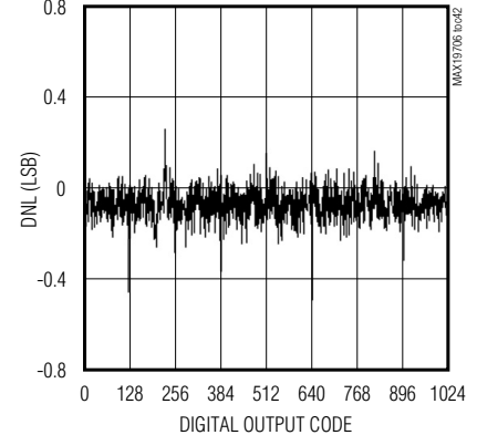
AUX-ADC DIFFERENTIAL NONLINEARITY
