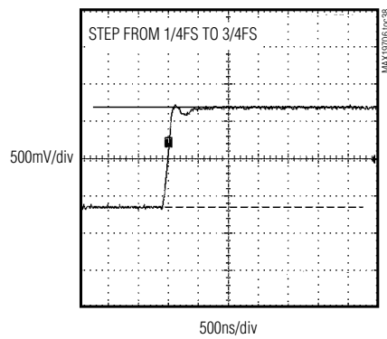
AUX-DAC SETTLING TIME
