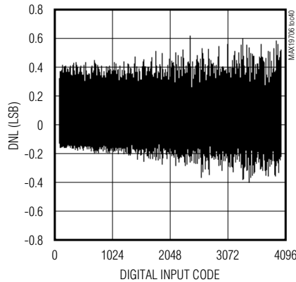
AUX-DAC DIFFERENTIAL NONLINEARITY
