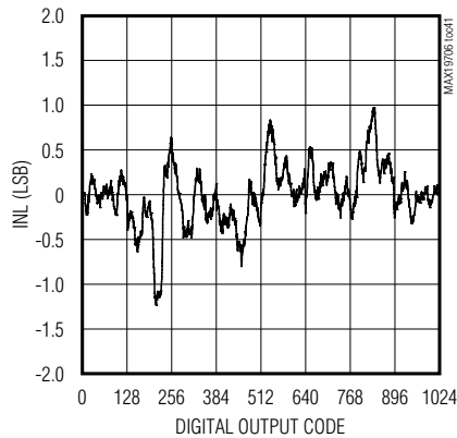
AUX-ADC INTEGRAL NONLINEARITY
