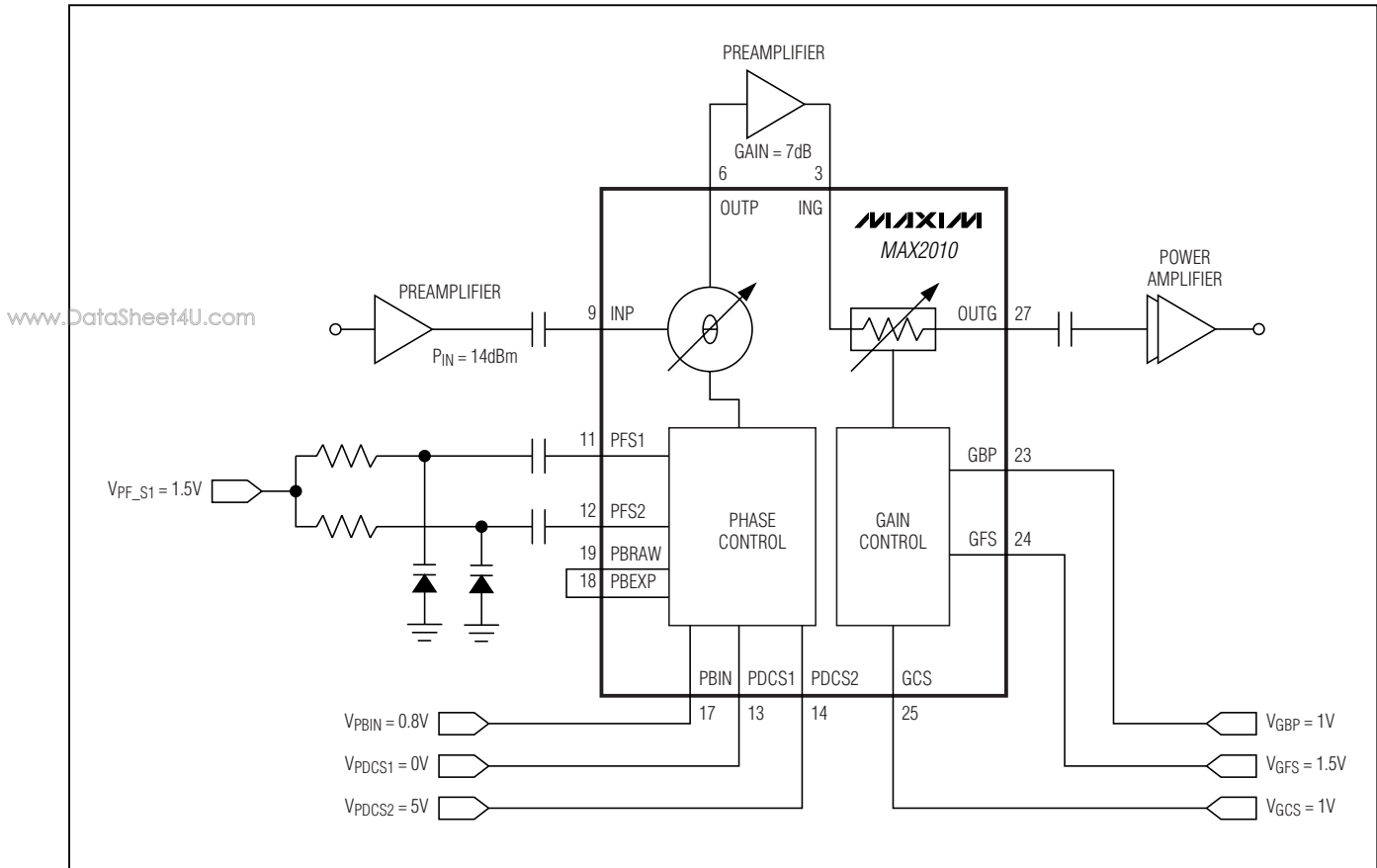
Figure 5. MAX2010 Phase and Gain Optimization Circuit
