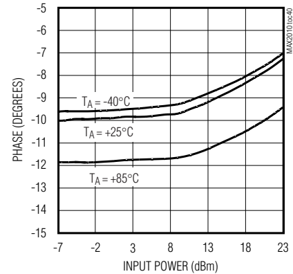
PHASE EXPANSION vs. INPUT POWER
