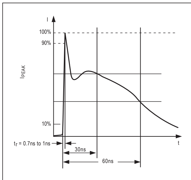
Figure 7b. IEC1000-4-2 ESD Generator Current Waveform
