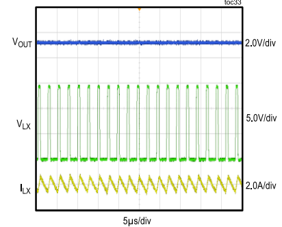
STEADY-STATE SWITCHING WAVEFORM (MAX20406AFOB)
