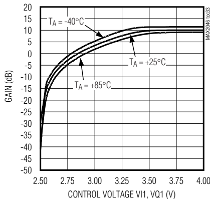
GAIN vs. CONTROL VOLTAGE (V1 = VQ1)
