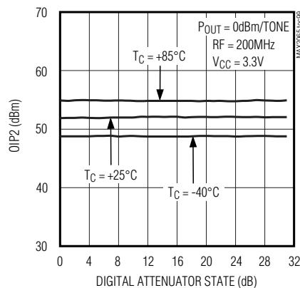
OIP2 vs. DIGITAL ATTENUATOR STATE
