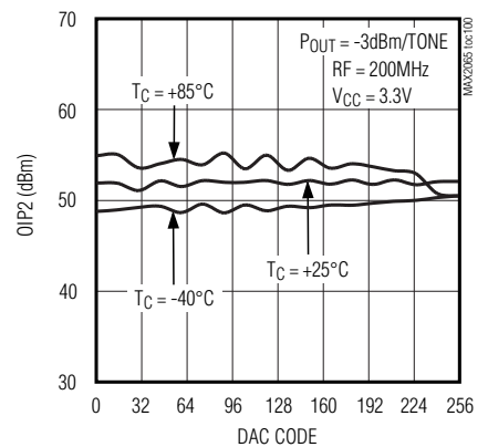
OIP2 vs. ANALOG ATTENUATOR STATE
