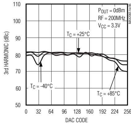
3rd HARMONIC vs. ANALOG ATTENUATOR STATE
