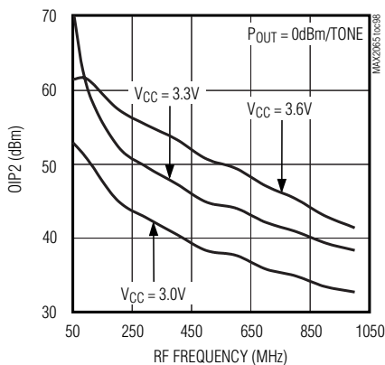
OIP2 vs. RF FREQUENCY
