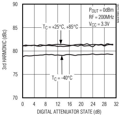
3rd HARMONIC vs. DIGITAL ATTENUATOR STATE
