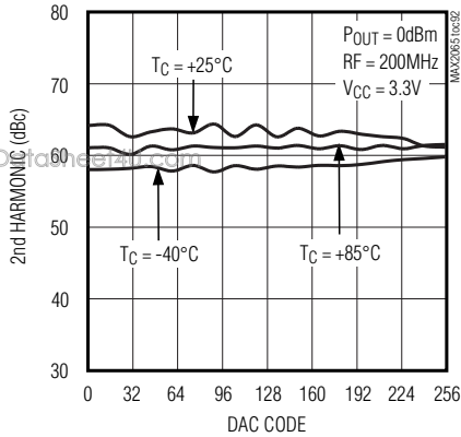
2nd HARMONIC vs. ANALOG ATTENUATOR STATE
