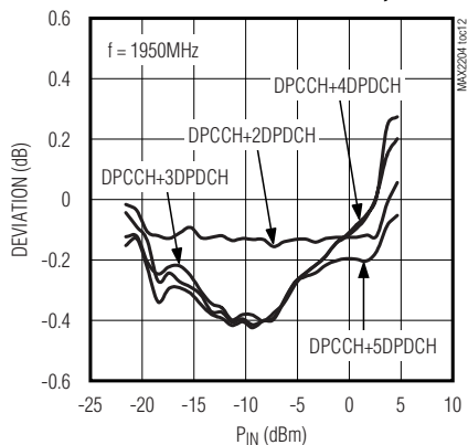
DEVIATION FROM DPCCH+1DPDCH, 1950MHz
